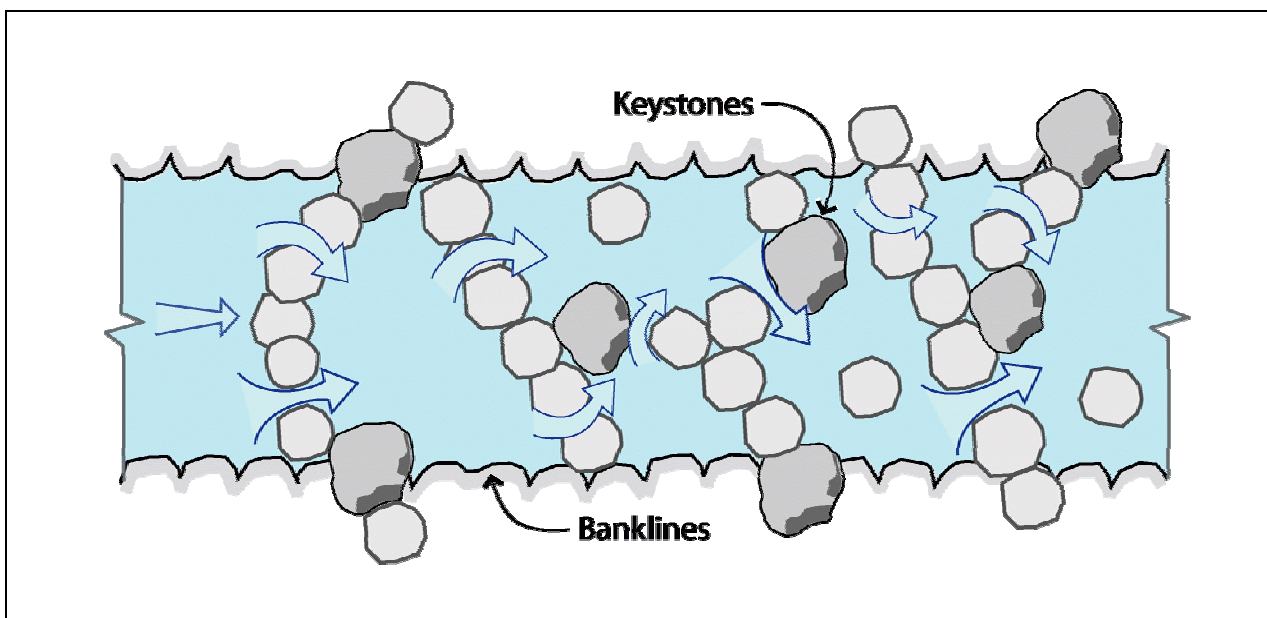
Figure XII-25. Cascade subunit of a cascade and pool channel. The cascade is a complex series of small steps form numerous pathways for fish to swim during lower flows while creating a rough cascade at higher flows.
