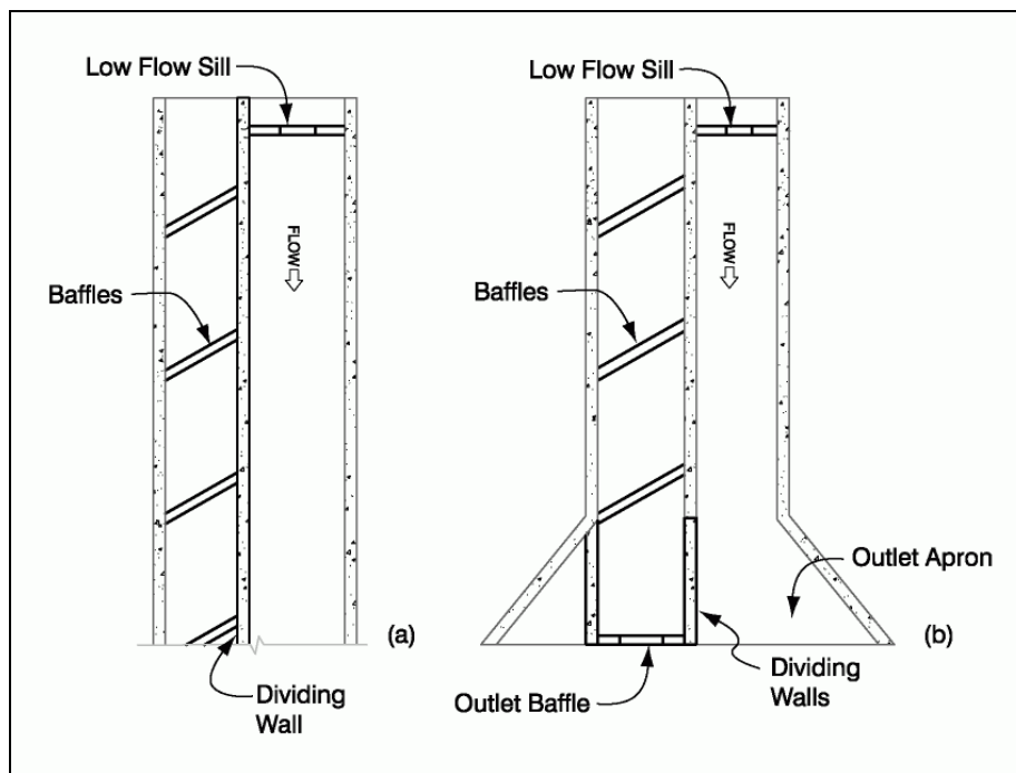
Figure XII-40. Dividing walls used (a) to baffle one side of a wide culvert and (b) to confine the flow on an outlet apron. The low-flow sill provides flow control to concentrate lower flows into the baffled section.
