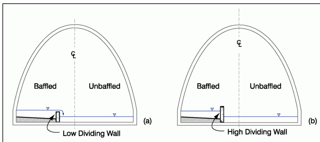
Figure XII-41. Section views of a wide culvert with (a) low and (b) high dividing walls that separate the baffled and un-baffled sections. Before overtopping the dividing wall, the baffled section should contain enough flow to generate sediment scouring forces.
