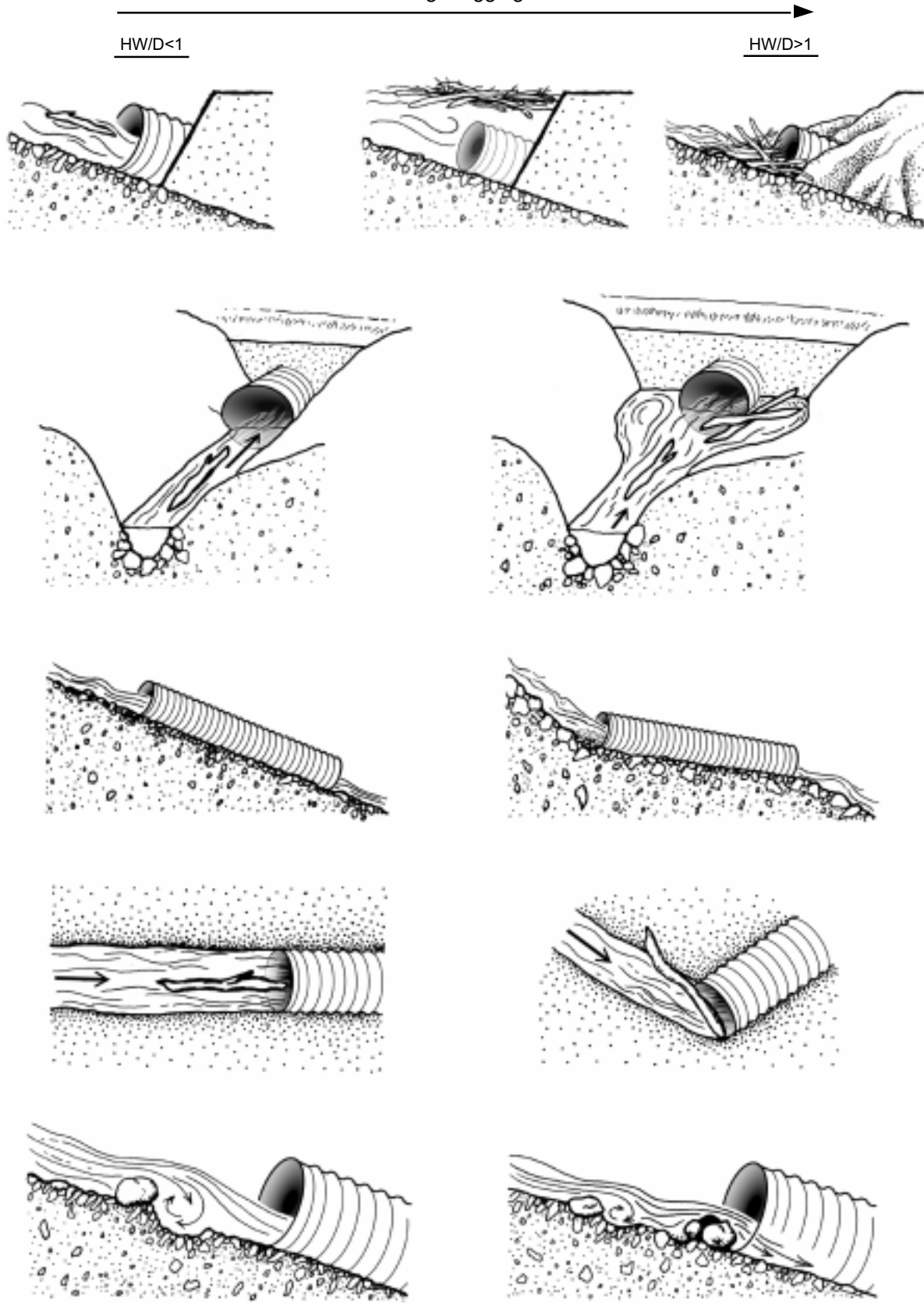
Figure 11—Illustrations of increasing plugging hazard.
